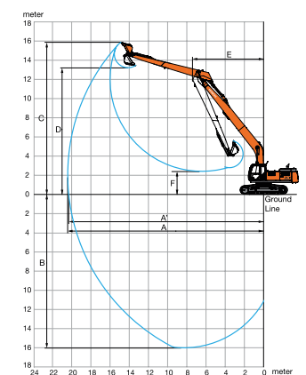
Mod. ZX300 LCN-6 LONG REACH
