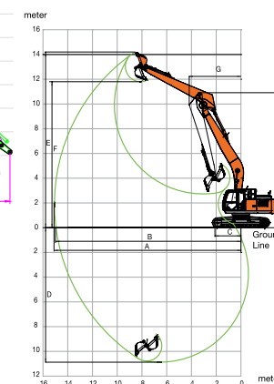
Mod. ZX210 LCN-5 LONG REACH
